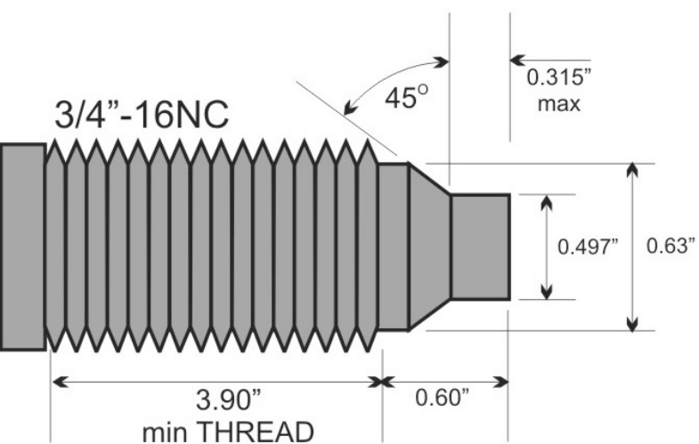
3/4"-16NC STANDARD
