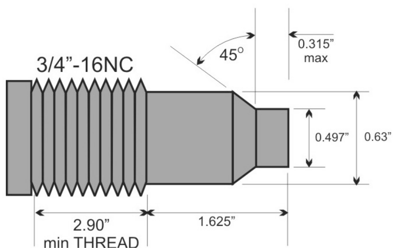
3/4"-16NC RECESSED
